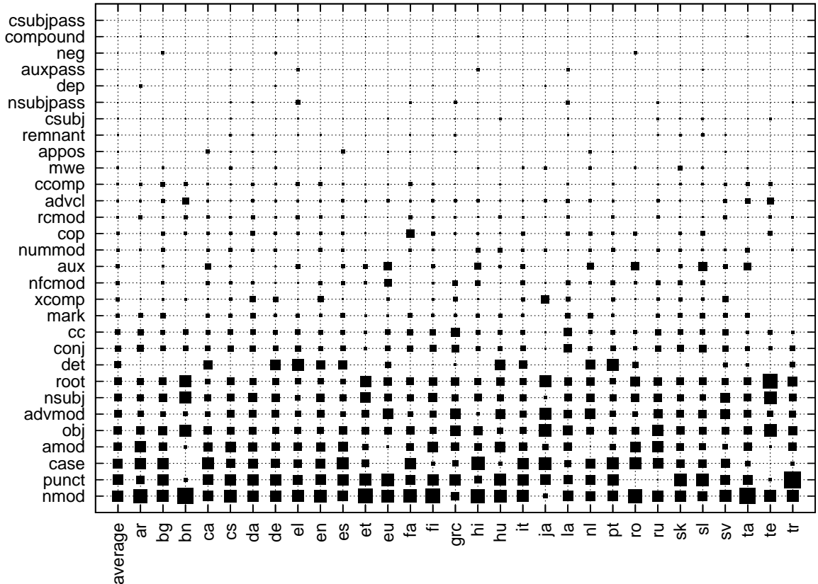
Figure 5: Distribution of USD labels in all the 30 HamleDT treebanks after stanfordization. The area of each square corresponds to the proportion of the given label in the given language.
