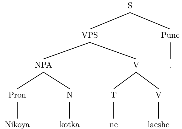
Figure 1: Sample tree of Example 1 from BTB
